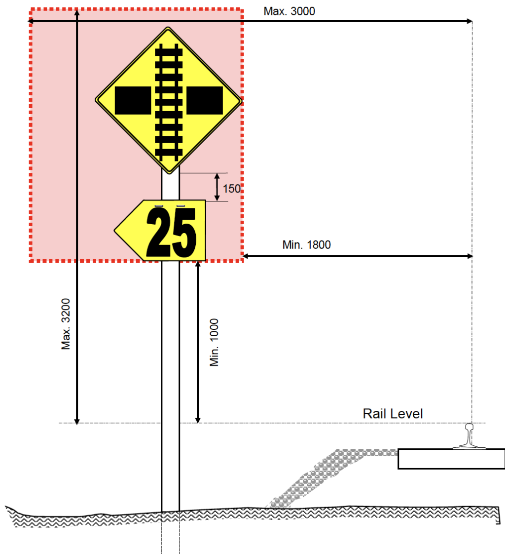
Figure 14 - Placement envelope for level crossing speed signs
