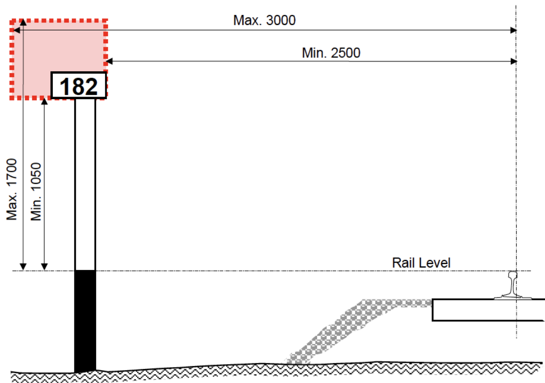
Figure 17 - Lateral placement of kilometre posts
