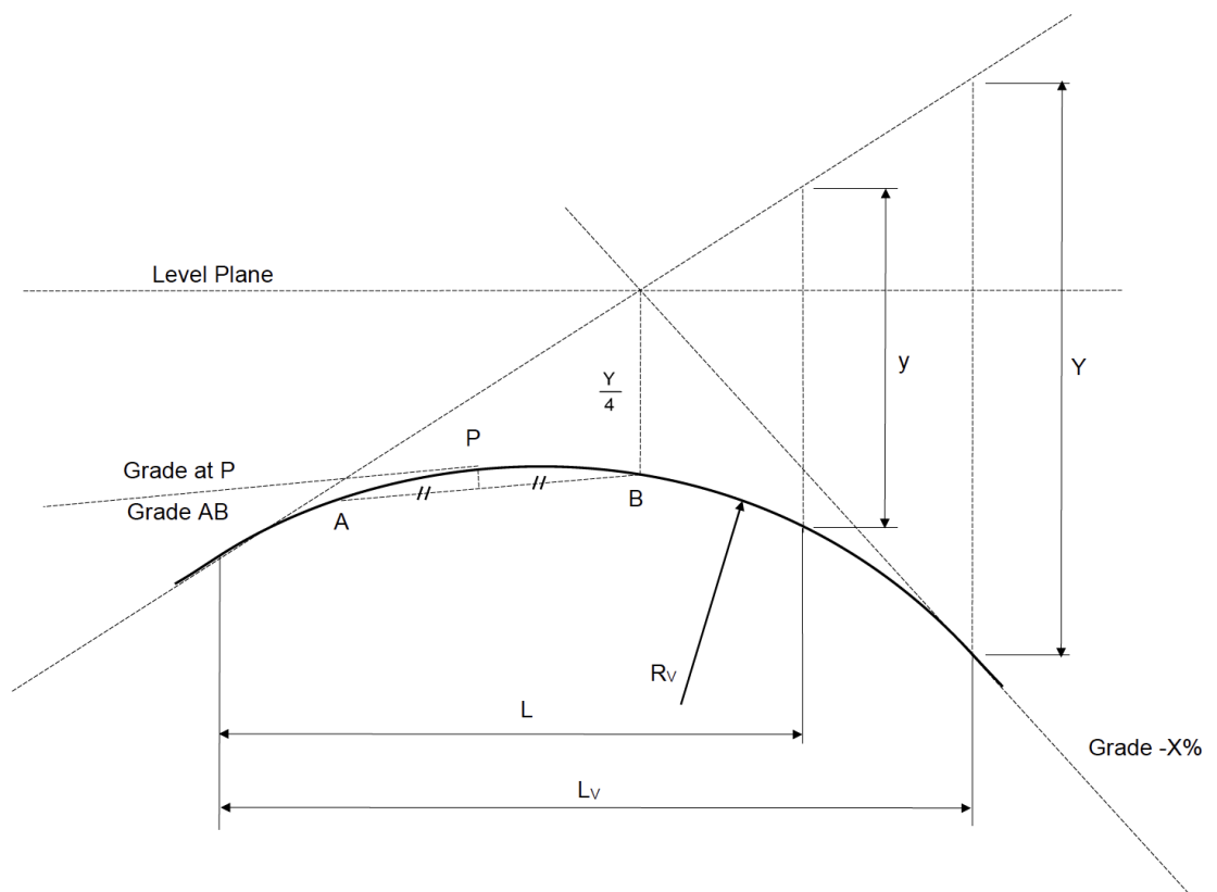
Figure 9 - Vertical curve component
