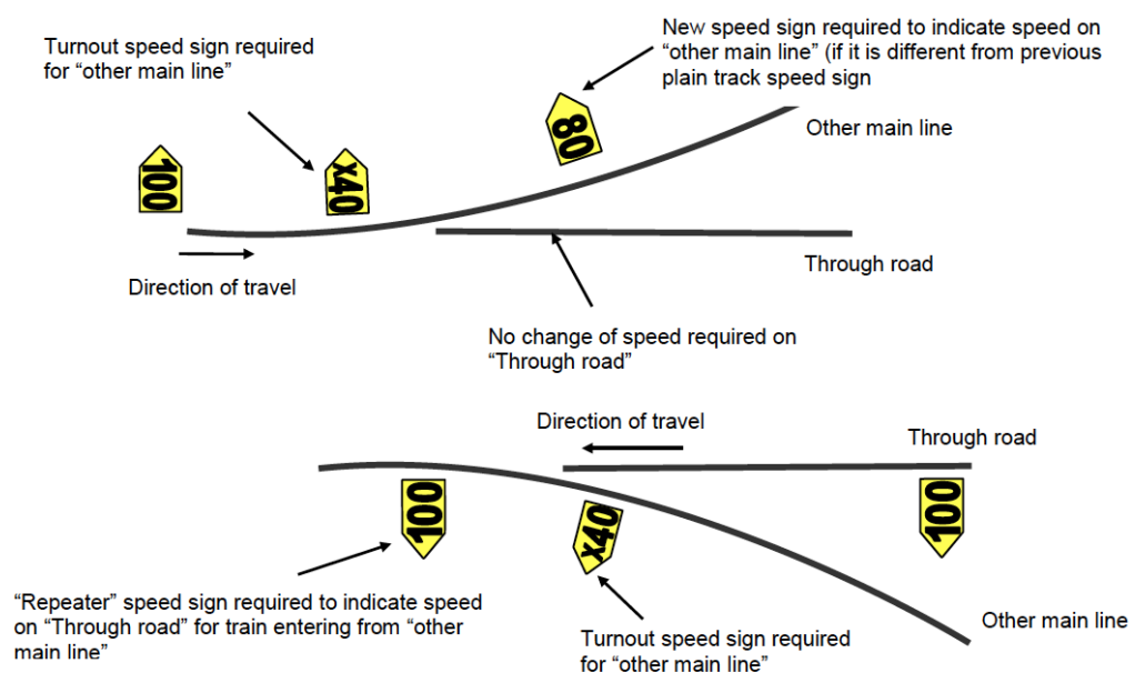
Figure 12 - Example of speed sign layout for converging/diverging roads
