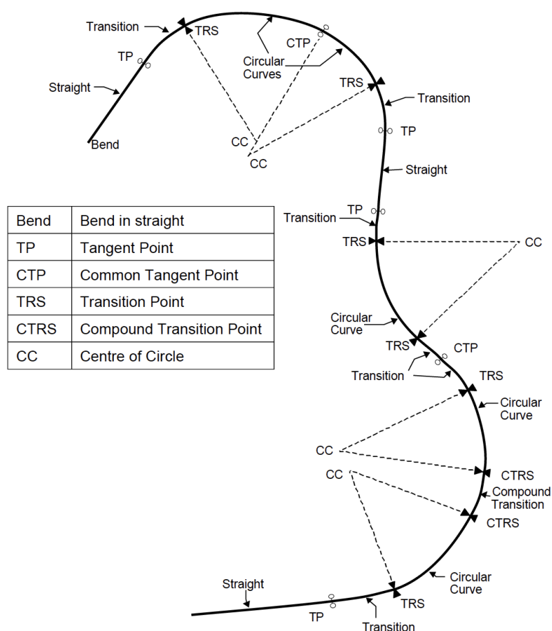
Figure 1 - Horizontal alignment component combinations
