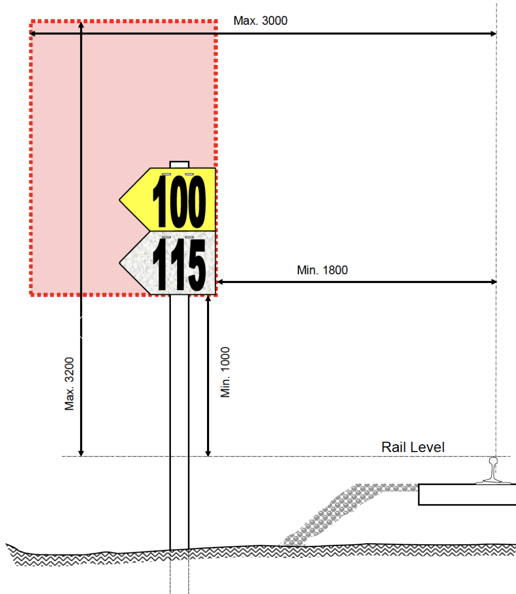
Figure 13 - Placement envelope for permanent speed signs
