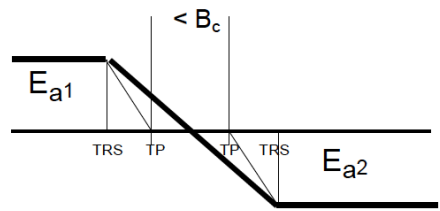
Figure 10 - Methods of applying superelevation
