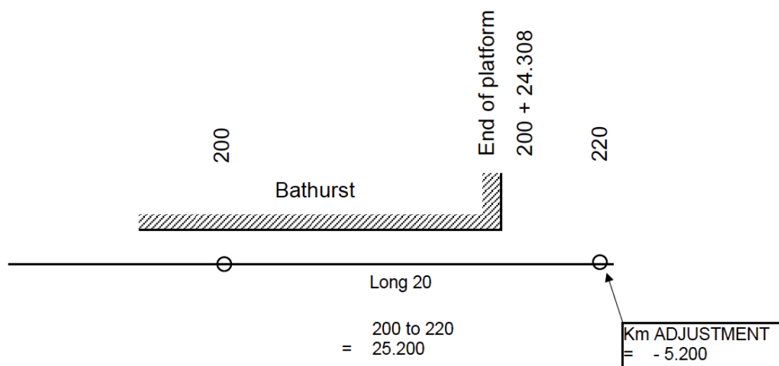
Figure 7 - Long kilometrage adjustment
