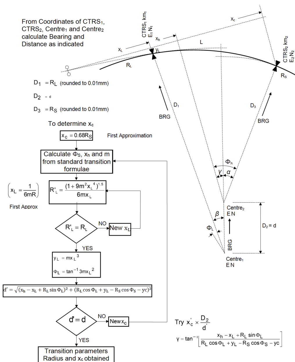
Figure 6 - Compound transition component
