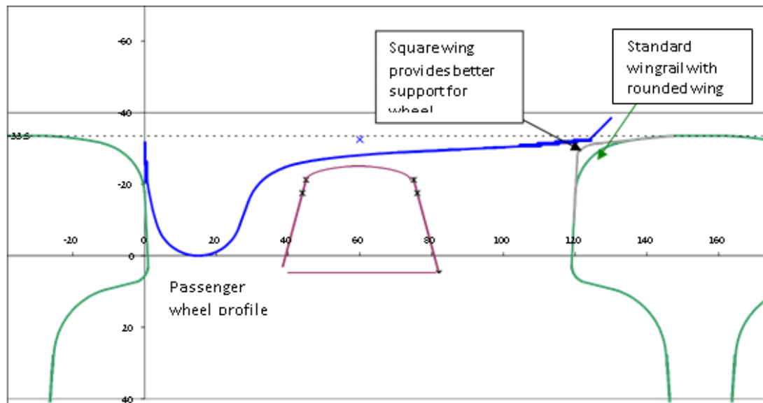
Figure 32 – Cross-Section showing square vs rounded wing
