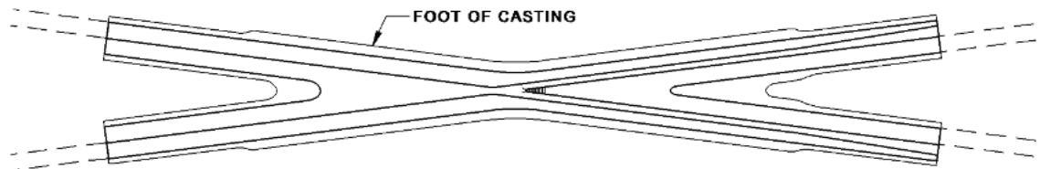
Figure 13 - 'V' Crossing Types - Solid Cast Manganese Crossing
