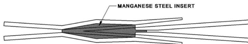
Figure 14 - 'V' Crossing Types - Rail Bound Manganese Crossing
