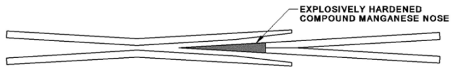
Figure 11 - 'V' Crossing Types - Compound Manganese Nose Crossing
