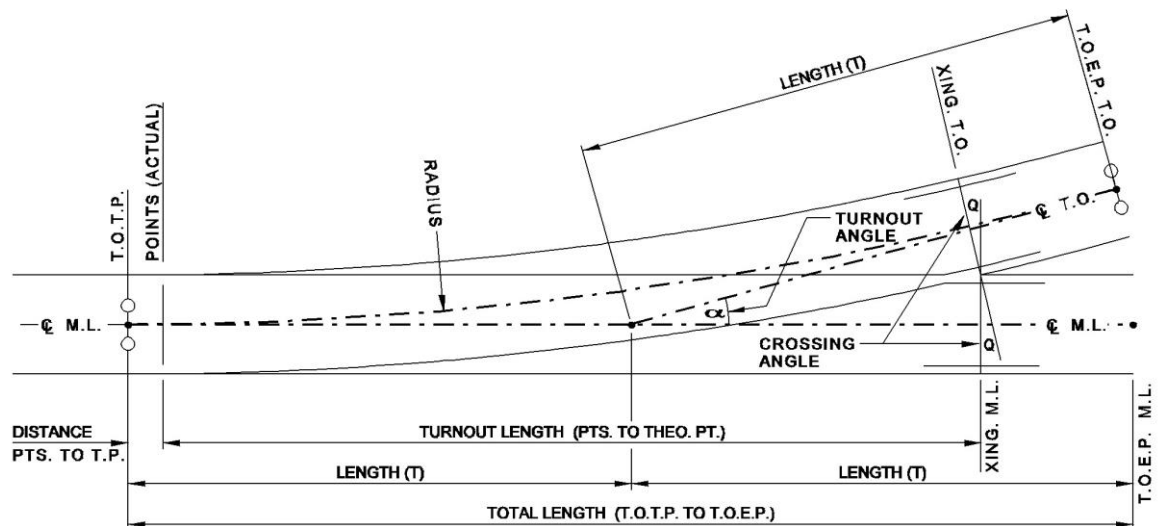
Figure 30 - Curved Crossing Turnout (drawn for LH turnout)
