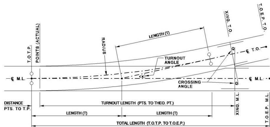
Figure 29 - Straight Crossing Turnout (drawn for LH turnout)
