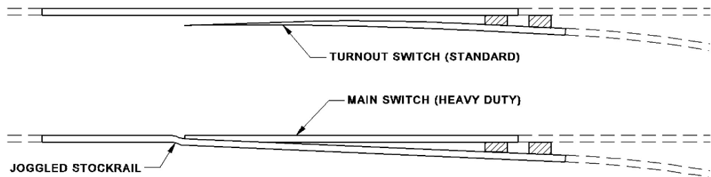
Figure 24 - Heavy Duty Switches
