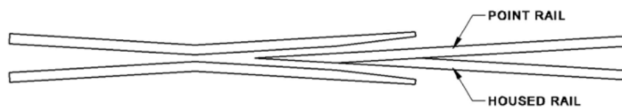
Figure 10 - 'V' Crossing Types - Fabricated Crossing Drawn for R.H. point rail
