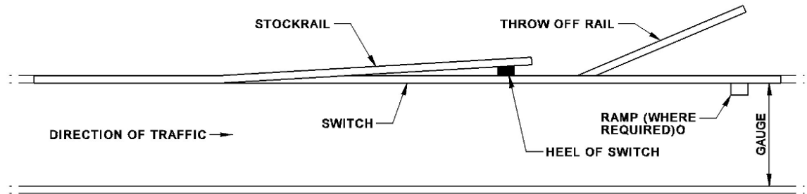
Figure 26 - Catchpoint Configuration
