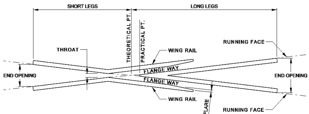
Figure 9 - 'V' Crossing Types - 'V' Crossing
