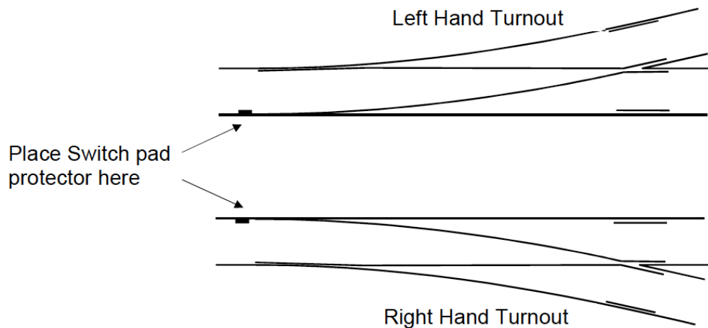
Figure 6 - Location of switch pad protectors
