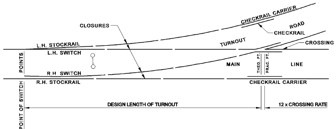
Figure 8 - 'V' Crossing Types - Standard Turnout Configuration (Drawn for L.H. Turnout)
