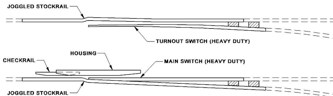
Figure 25 - Housed Switches
