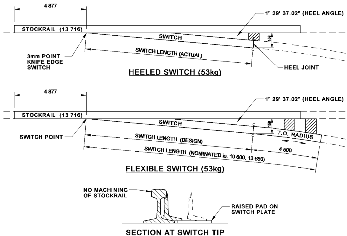
Figure 17 - 53kg Heeled & Flexible Switches
