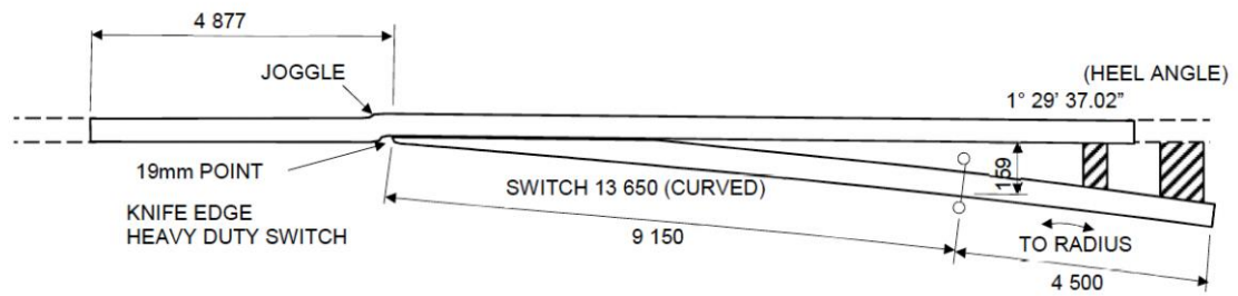
Figure 18 - 13 650 Heavy Duty Switch, 159 Heel (53kg)
