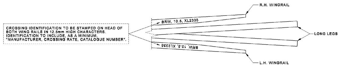
Figure 16 - Current requirement (To be retained)
