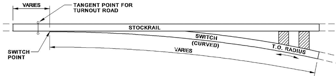
Figure 22 - 50kg & 60kg Tangential Switch
