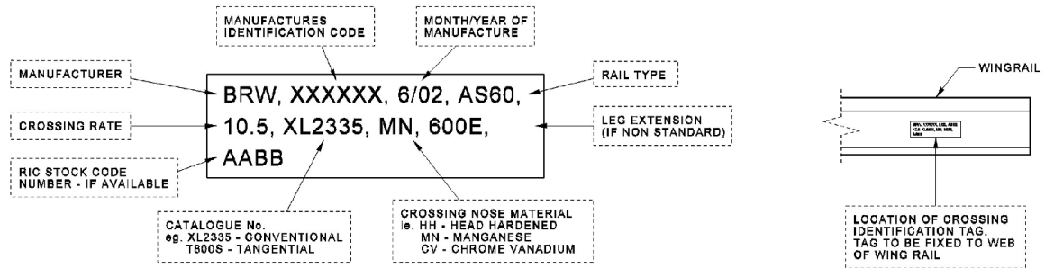
IDENTIFICATION TAG (CONTAINS A MINIMUM OF " MANUFACTURER, DATE OF MANUFACTURE, RAIL TYPE, CROSSING RATE, CATALOGUE NUMBER")
