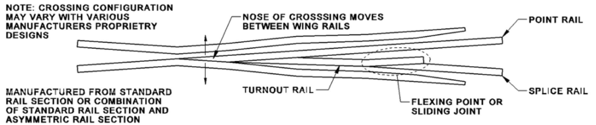
Figure 12 - 'V' Crossing Types - Fabricated Swing Nose Crossing
