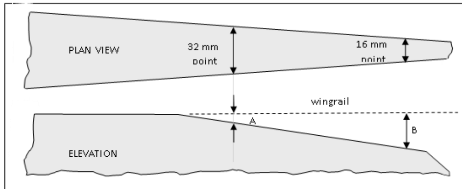
Figure 31 – Crossing nose design slope
