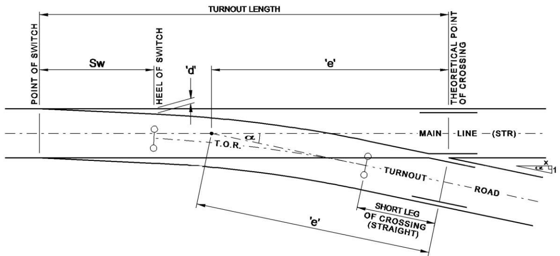
Figure 27 - Straight Crossing Conventional Turnout (drawn for RH turnout)
