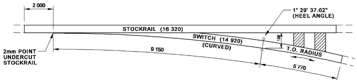
Figure 20 - 9 150 Flexible Switch
