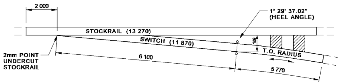
Figure 19 - 6 100 Flexible Switch
