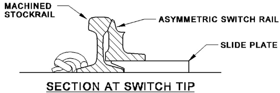
Figure 23 - Tangential Switches
