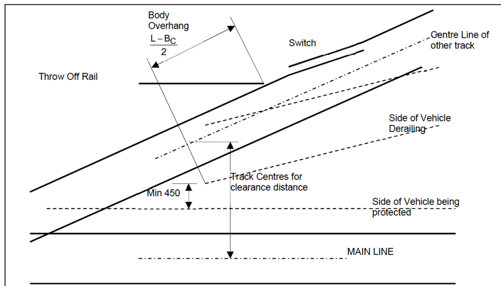
Figure 5 - Clearances at Catchpoints
