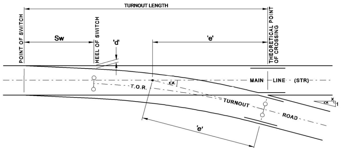
Figure 28 - Curved Crossing Conventional Turnout - short leg curved (drawn for RH turnout)
