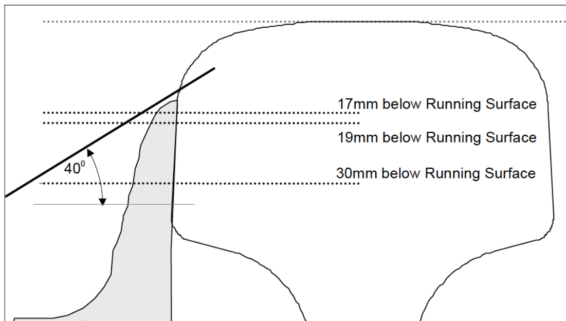
Figure 7 - Switch tip acceptance limits
