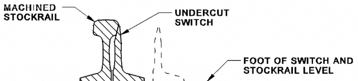
Figure 21 - Section at Switch Tip - 50kg & 60kg Flexible Switches
