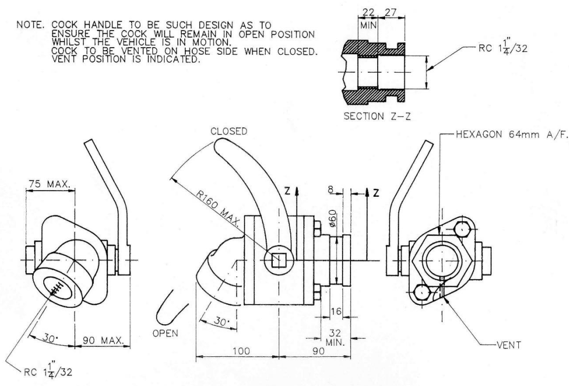
Figure 7 Brake pipe coupling cock
