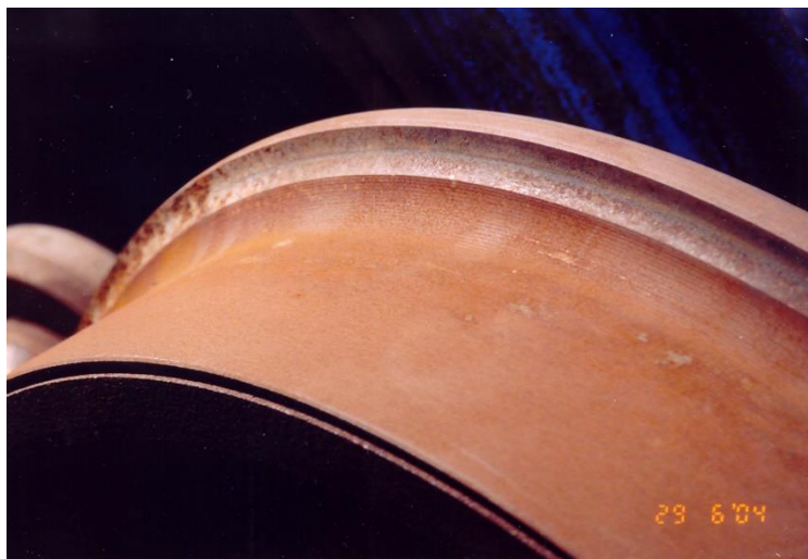
Figure 4 An unacceptable witness mark
