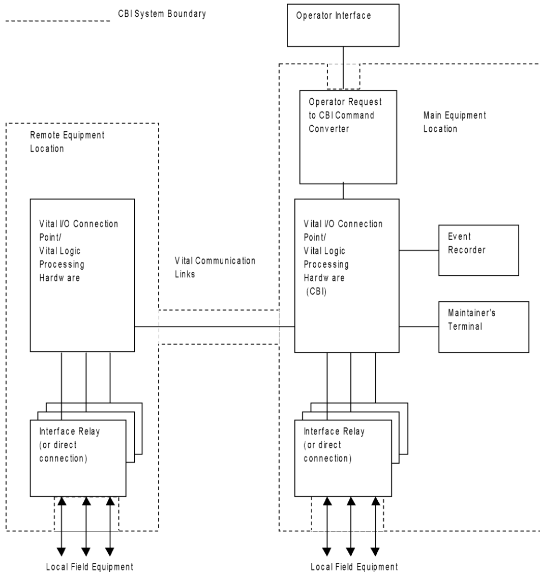
Figure 1 – The Operator Interface boundary
